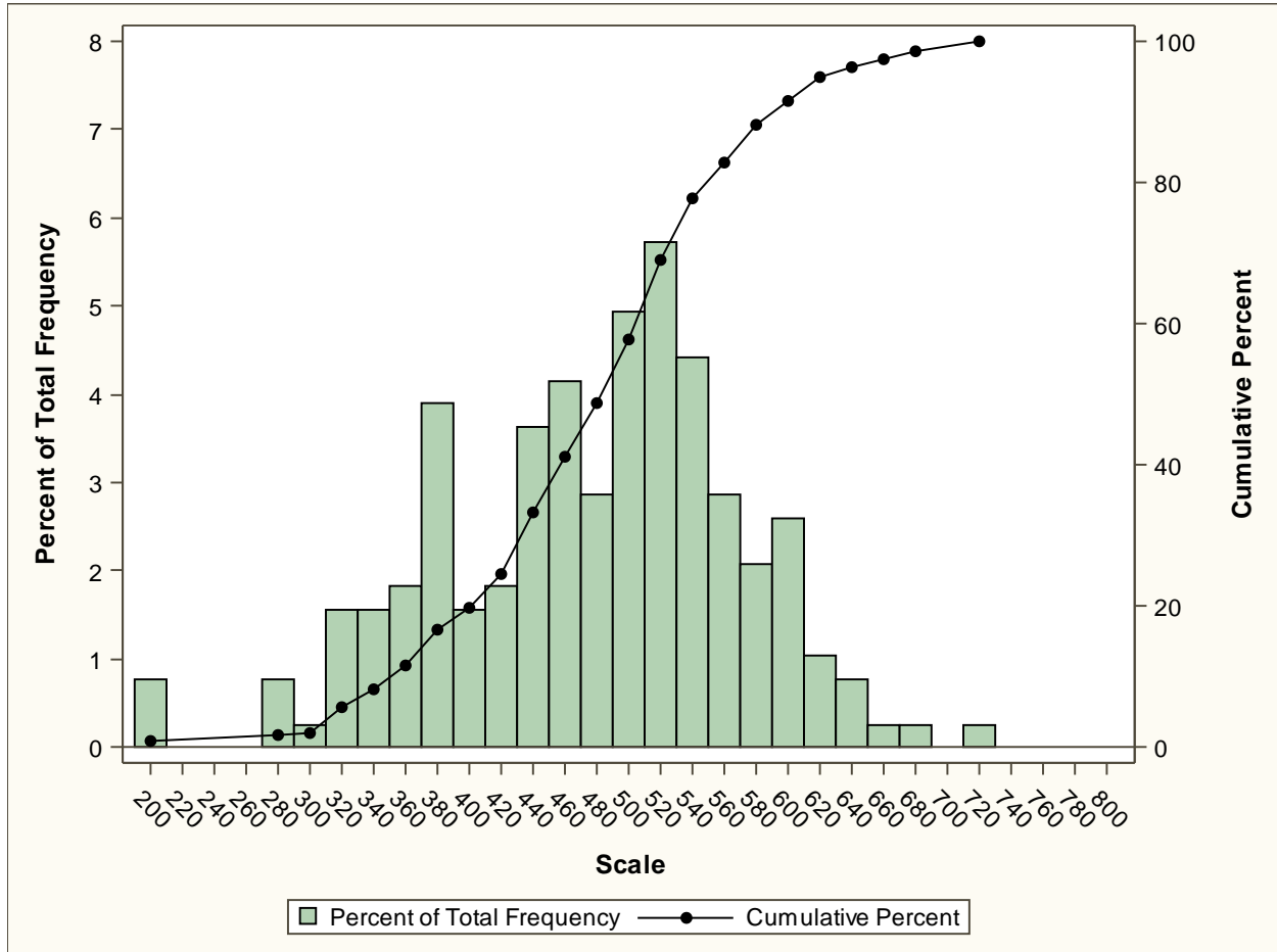
Frequency distribution for the Clinical Sciences scale: 2018 (385 administrations)
