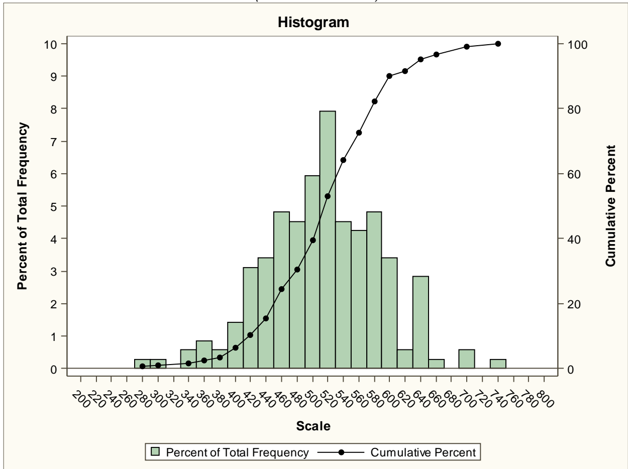
Frequency distribution for the ADAT Overall scale: 2016-2018 Orthodontics and Dentofacial Orthopedics (353 administrations)
