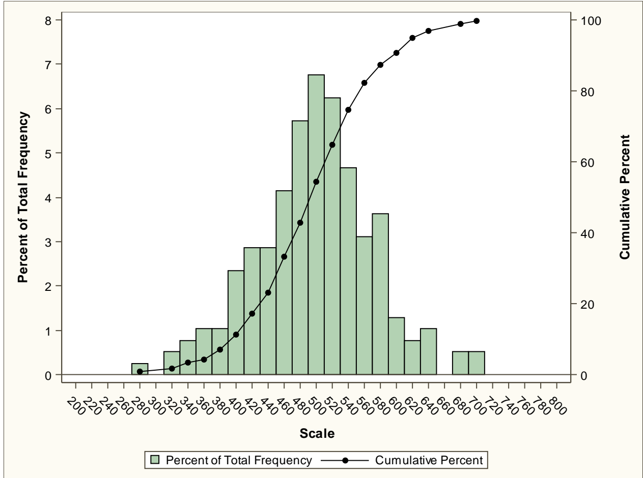
Frequency distribution for the ADAT Overall scale: 2018 (385 administrations)
