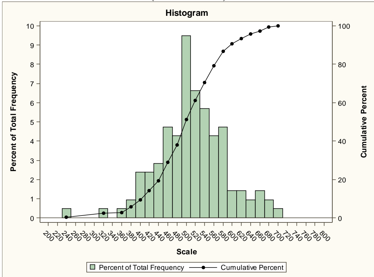
Frequency distribution for the ADAT Overall scale: 2016-2018 General Practice Residency, 12 Months (211 administrations)
