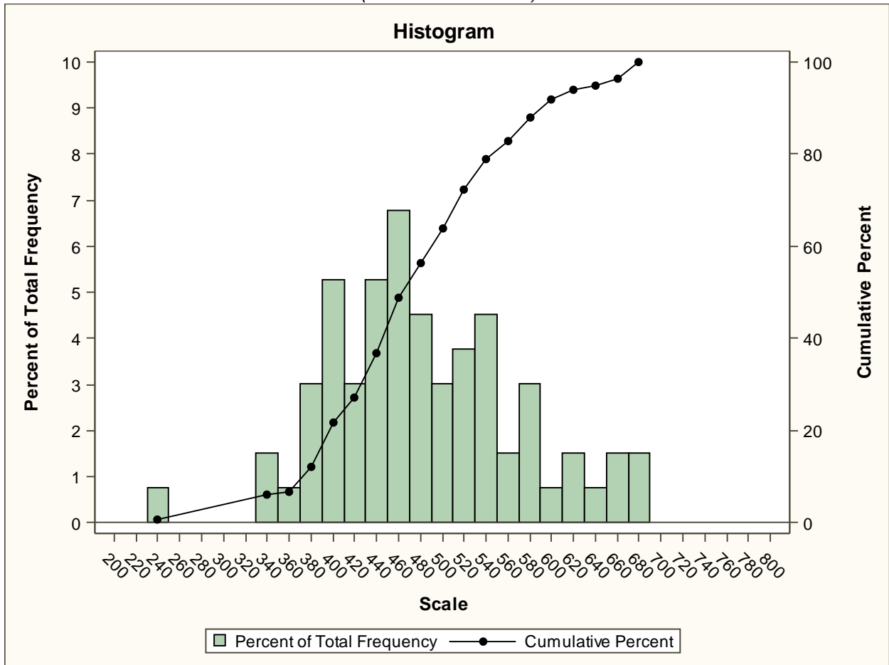
Frequency distribution for the ADAT Overall scale: 2016-2018 Advanced Education in General Dentistry, 24 Months (133 administrations)
